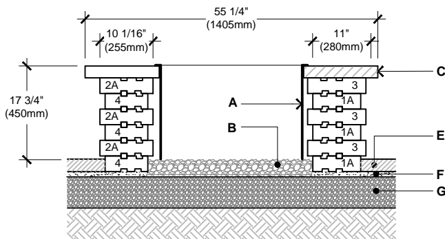
SECTION 1-1
